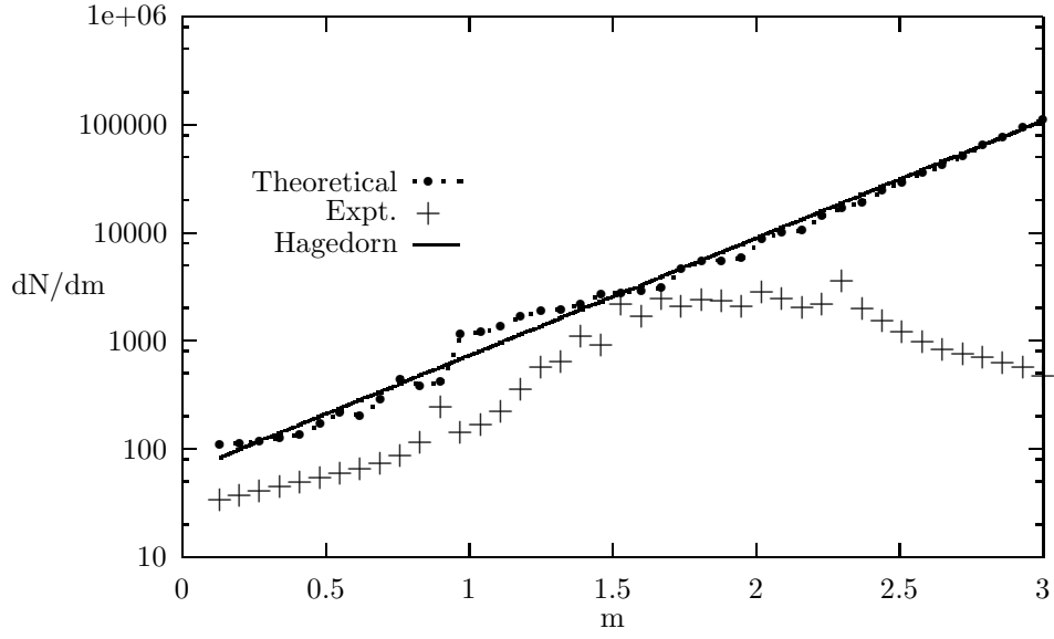
Figure 1: Comparison of experimental ('plus'-s, ++ ) and theoretically predicted density of states (dots .....). The straight line gives \sim \exp(m/T_H) .
